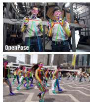
OpenPose [Chao 2019]
