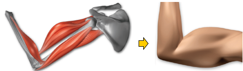
[Softimage XSI]
